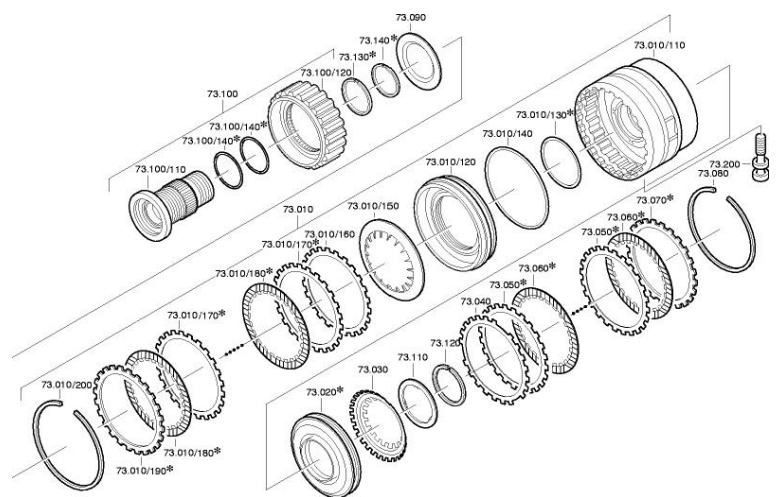
D-G Clutch
