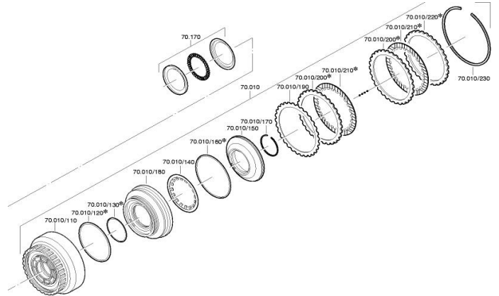
Clutch A
