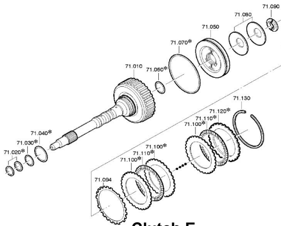
Clutch E
