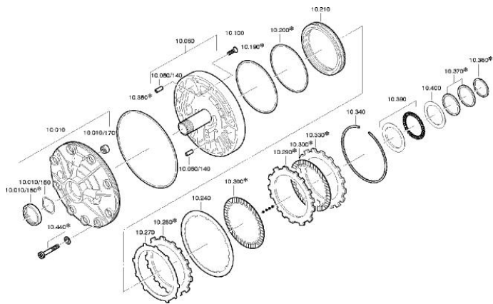
Oil Pump
